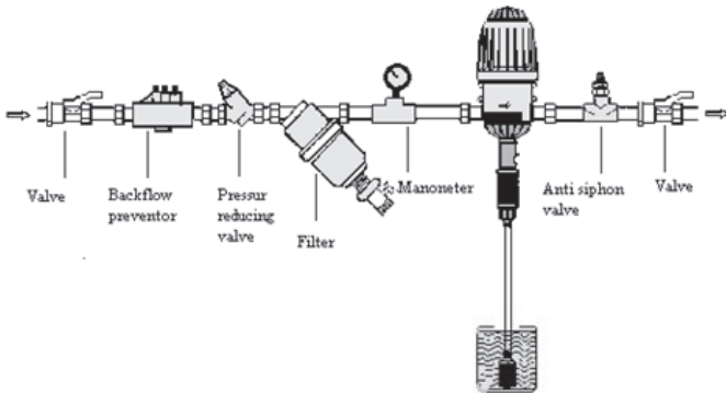
Correct Installation
